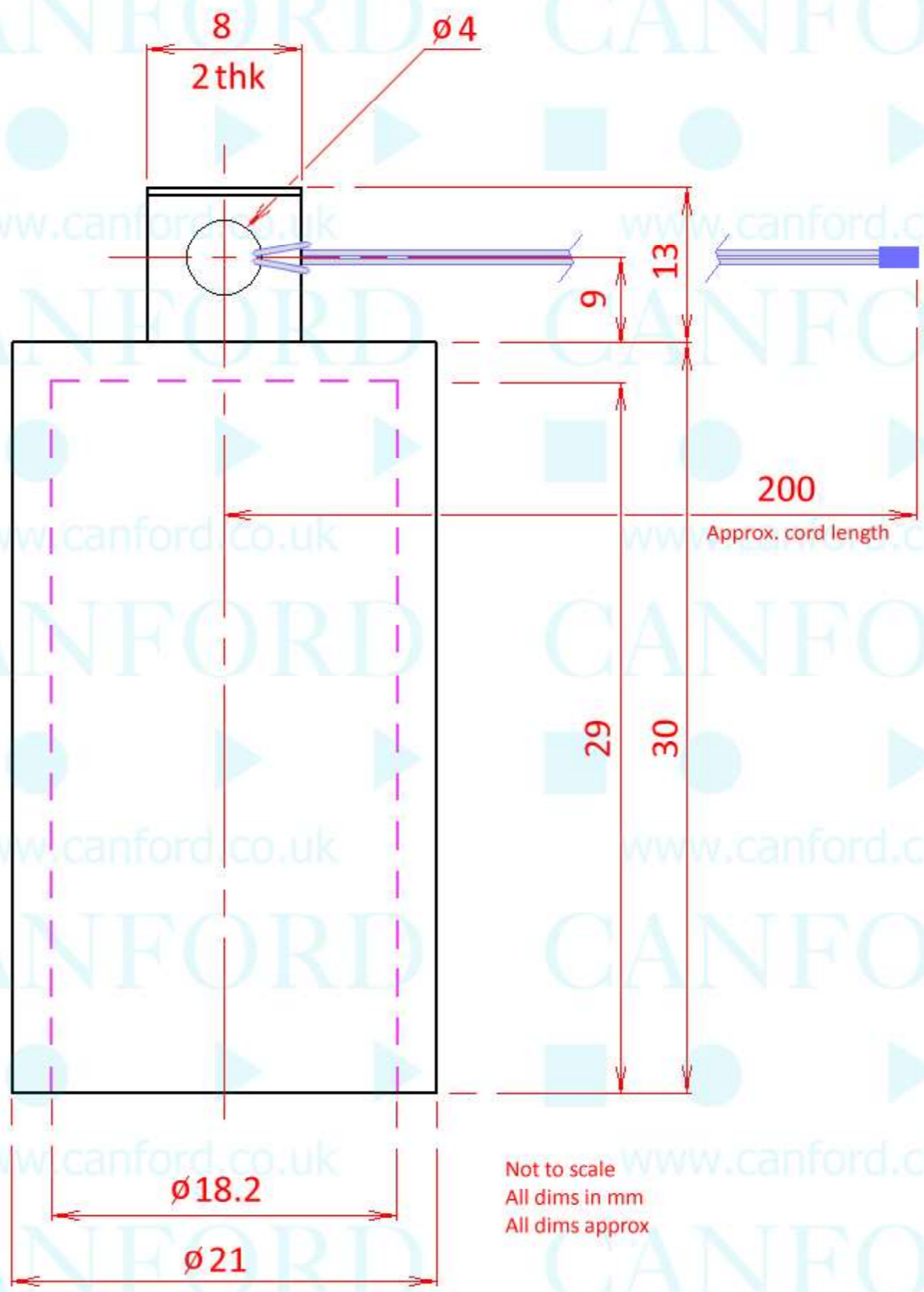
40-702 CANFORD CABLE CONNECTOR PROTECTIVE RUBBER CAP With cord
